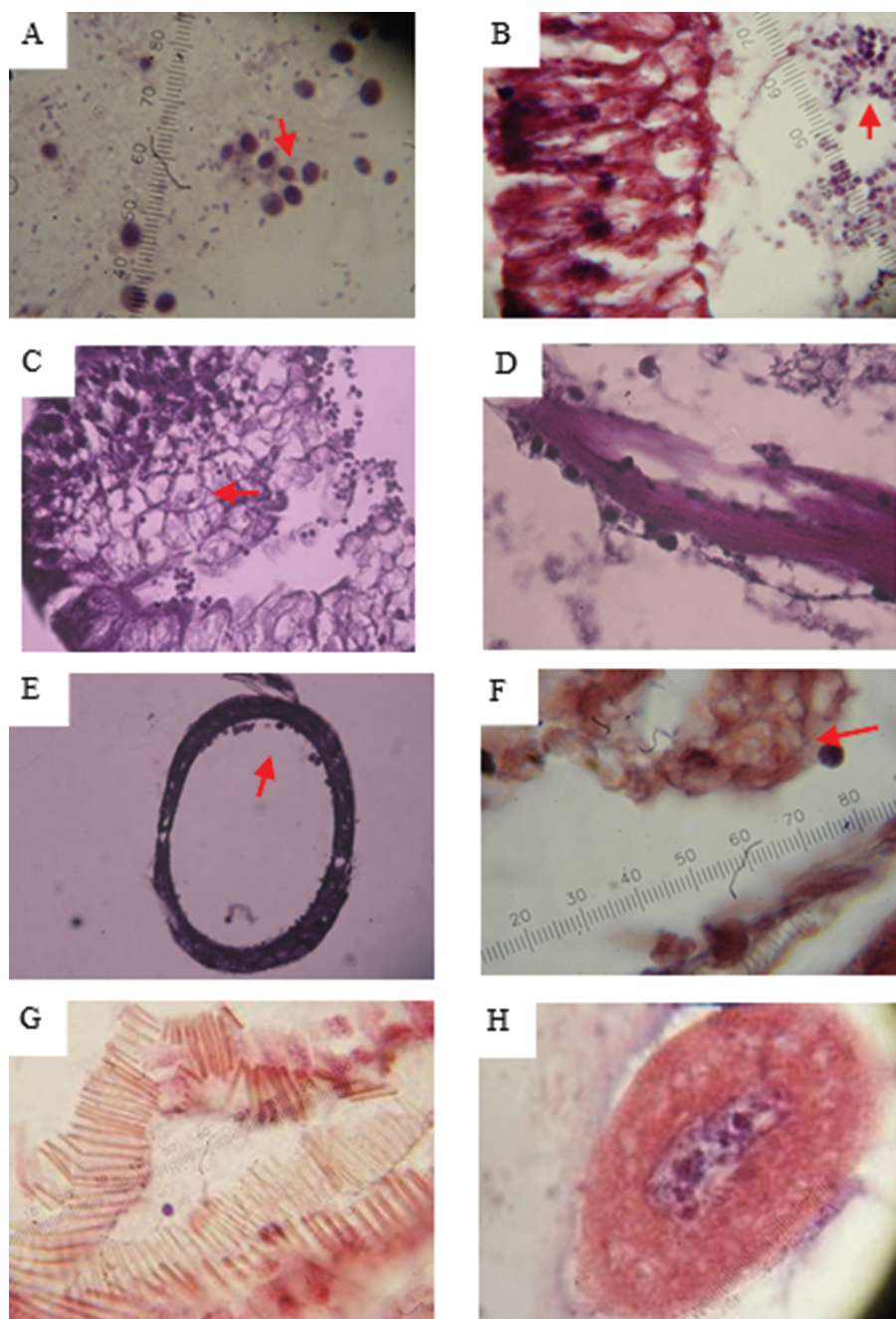
Fig. 1. PIBs SpltMNPV in: (A) Lumen midgut (1000×), (B) peritrophic membrane (400×), (C) midgut epithelium (400×), (D) muscle (1000×), (E) Malpighi tubules (400×), (F) fatty tissues (1000×), (G) trachea (1000×) and (H) blood vessels (100×).
